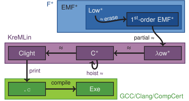
Fig. 3. The original Low^* -to-C translation
