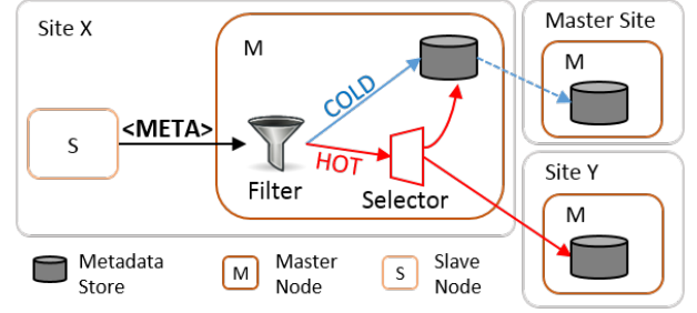
Fig. 3: The hot metadata filtering component.
