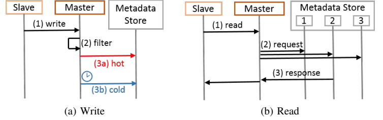
Fig. 5: Metadata Protocols.
