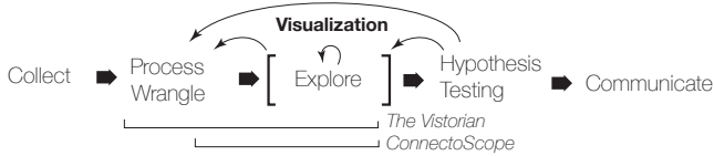
Figure 2: Exploration workflow
