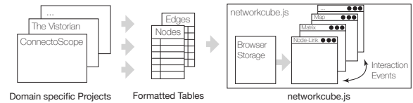
Figure 3: NetworkCube pipeline
