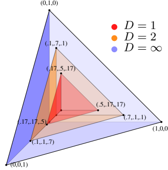
Fig. 3. Regions of d_Y -regular priors for Example 2
