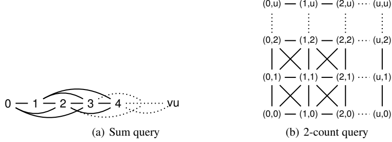
Fig. 5. Adjacency graphs
