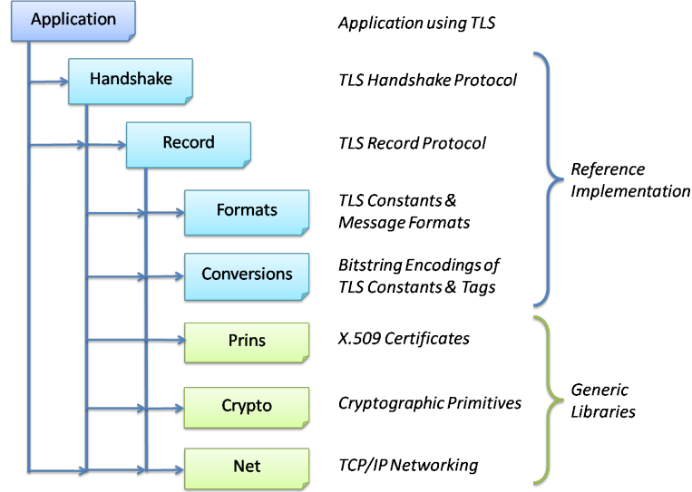
Fig. 2. Structure and Module Dependencies for our Implementation
